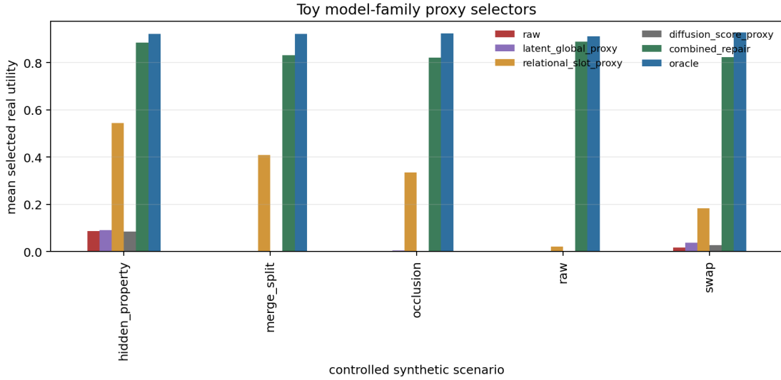
Figure 33: Toy model-family proxy diagnostics. These are controlled proxy selectors, not broad external benchmark comparisons.
