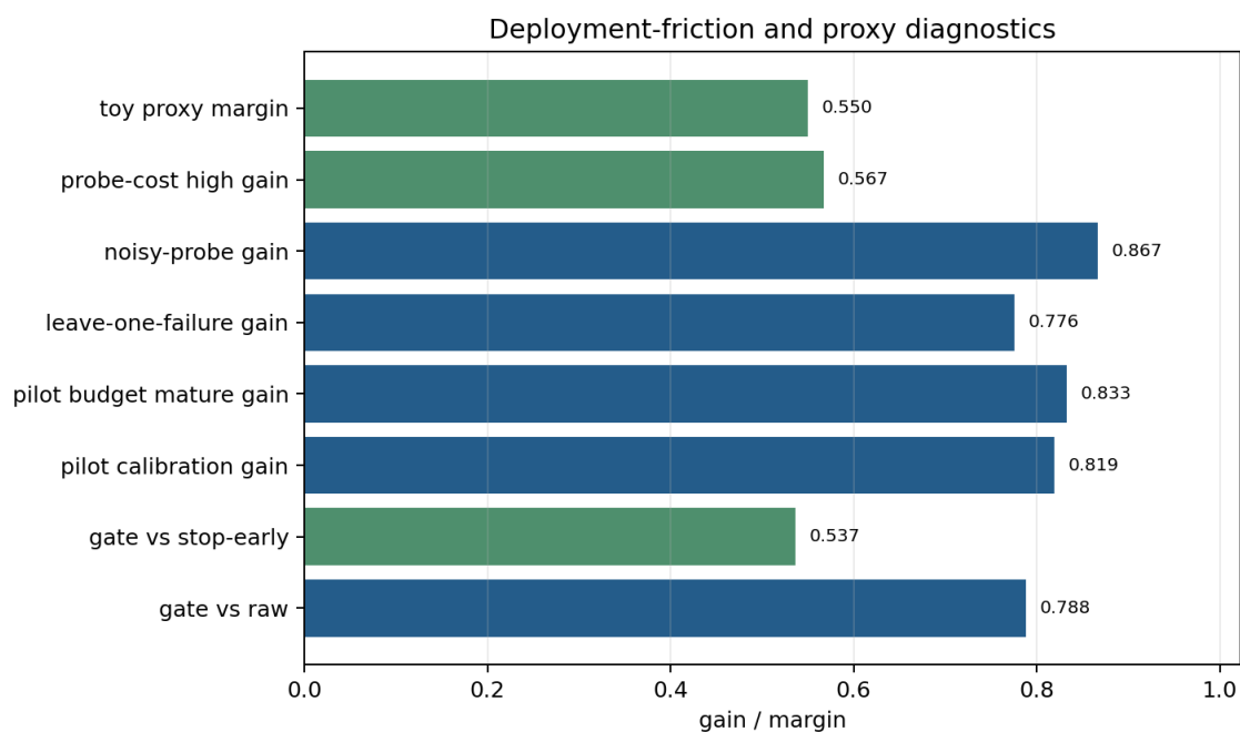
Figure 9: Deployment-friction diagnostics. Pilot labels, noisy probes, probe costs, deployment gating, and toy proxy comparisons are measured as controlled stress tests, not as external deployment evidence.
