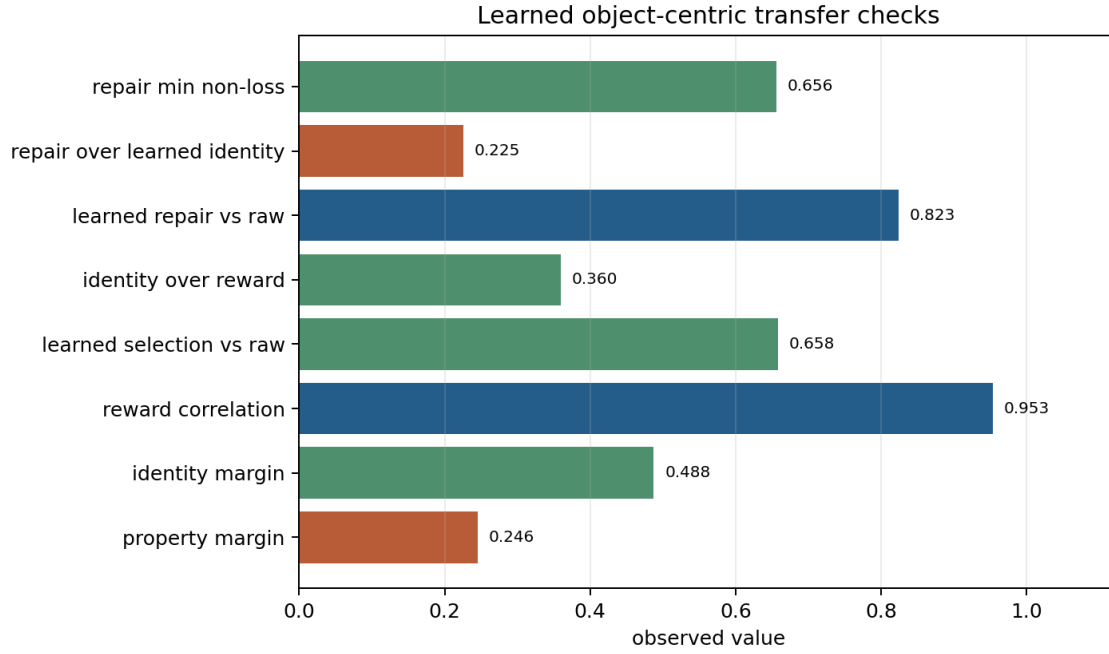
Figure 7: Learned object-centric transfer checks. Learned identity information improves selected-tail behavior, and the learned repair policy remains conservative relative to the learned identity+reward selector.
