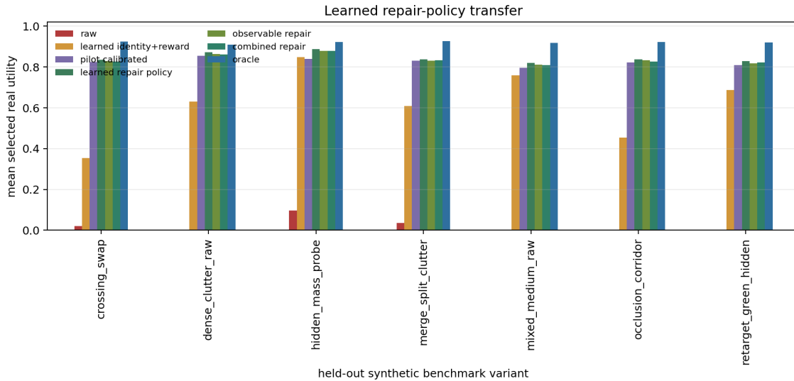
Figure 8: Learned repair-policy transfer. The policy uses observable diagnostics plus learned heads and is evaluated on held-out benchmark-style synthetic variants.
