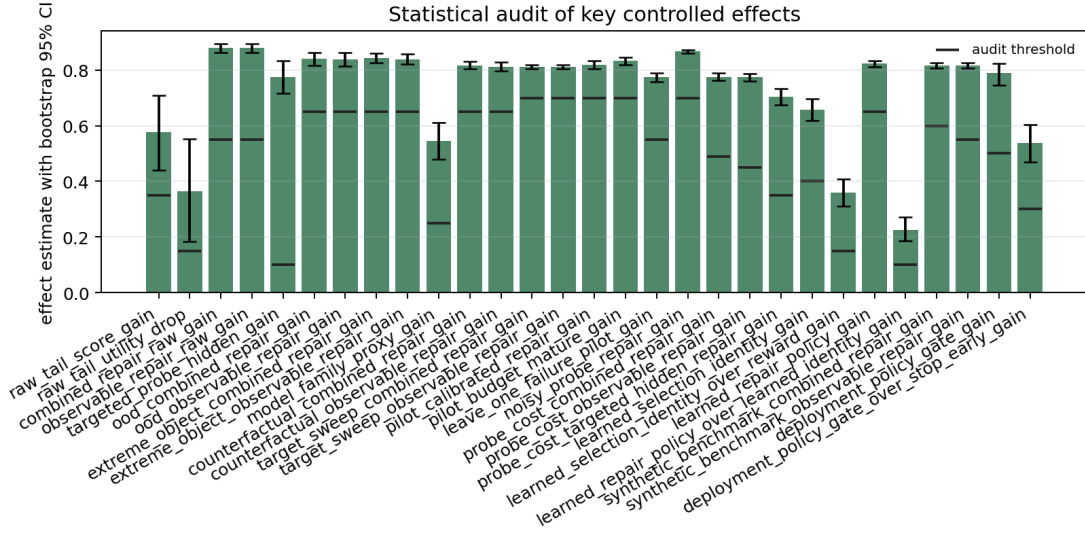
Figure 32: Bootstrap statistical audit.
