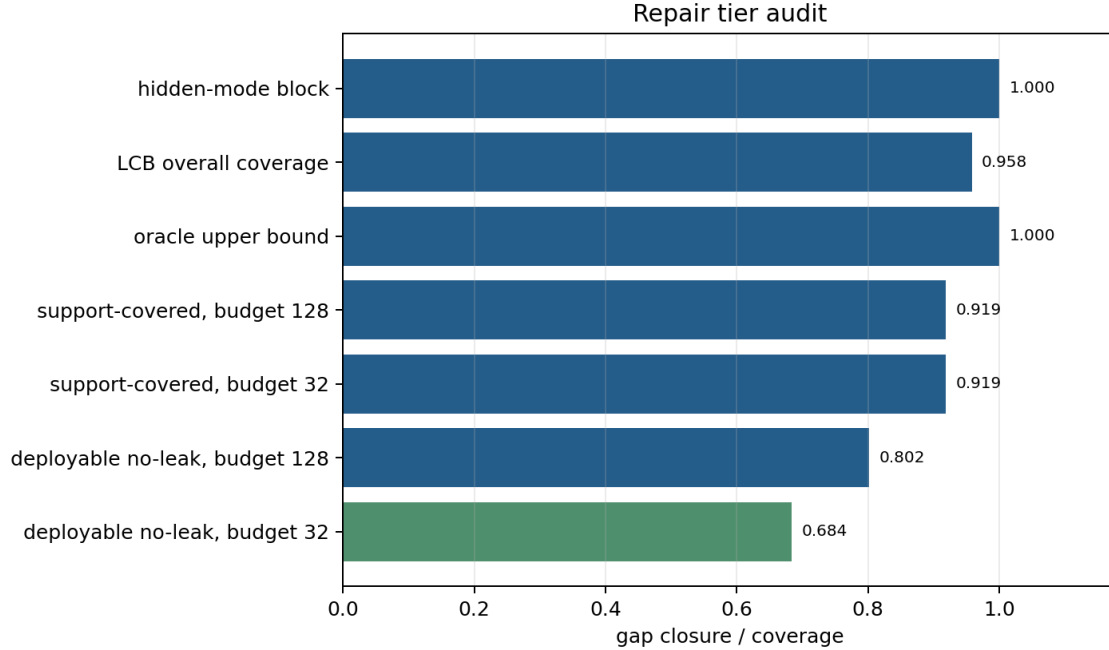
Figure 6: Repair tiers. The budget-32 no-leak row is useful but partial; support-covered and oracle rows are stronger but must not be treated as deployable proof.
