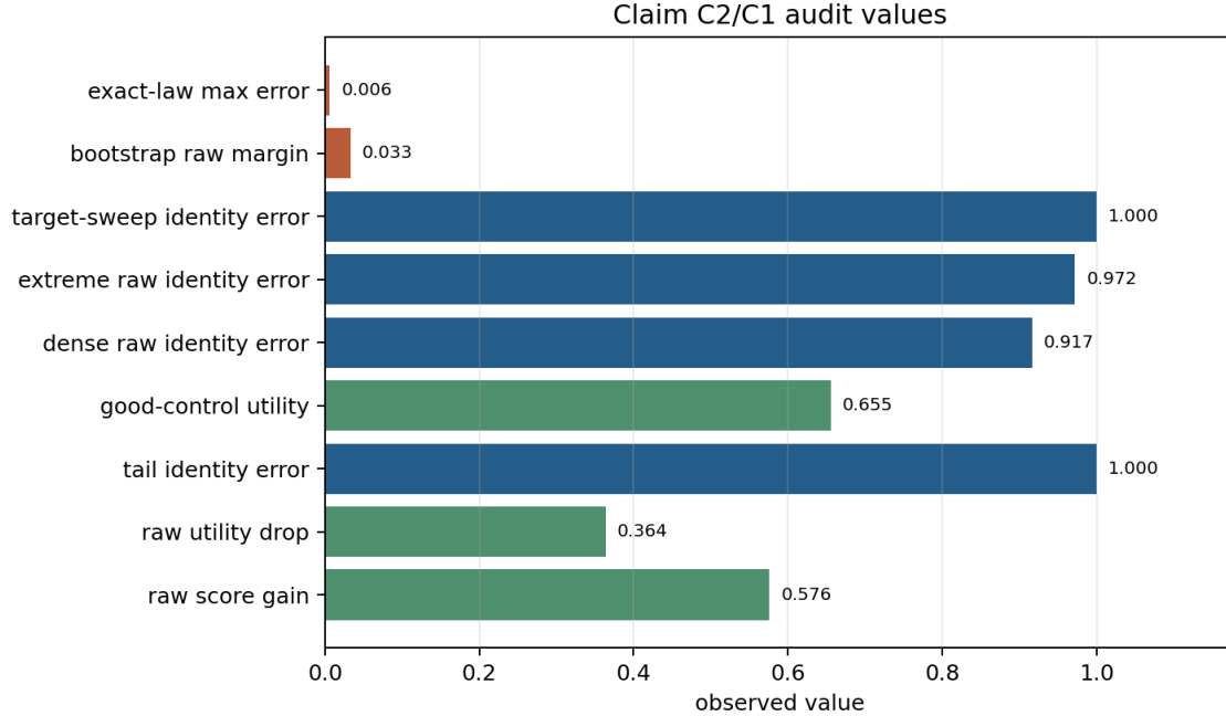
Figure 1: V3 evidence scorecard. The exact-law error is small; the dominant empirical signal is that raw high-budget selection increases score while producing severe identity error and lower real utility in corrupted object-centric scenes.
